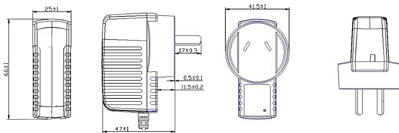
■ Dimension Diagram for KRE06SS-USB
