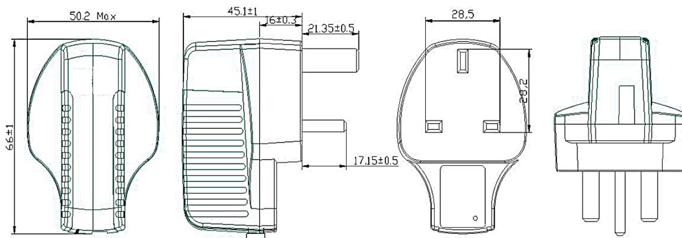
Dimension Diagram for KRE06SB-USB
