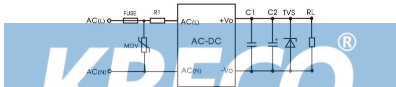
Fig. 2: EMC application circuit with higher requirements
