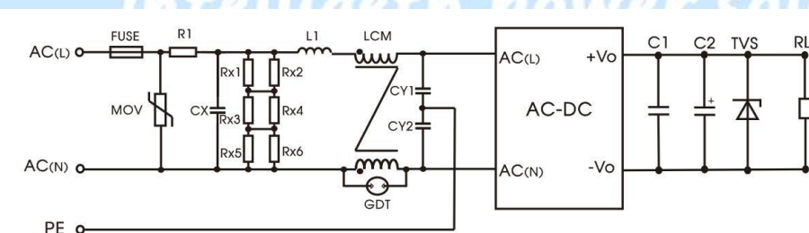
Fig. 3: Recommended circuit for class I equipment
