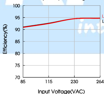
Efficiency Vs Input Voltage (Full Load)
